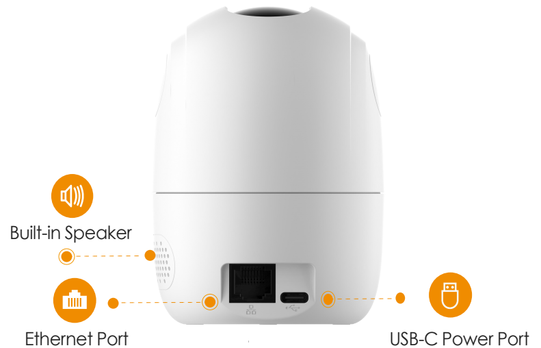
Back View
