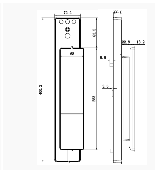
Front panel
