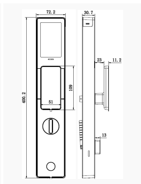
Rear panel for 5085
